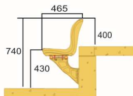
Riser Mounting
