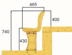
Floor Mounting
